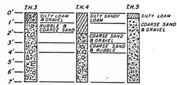
SOIL PROFILE
